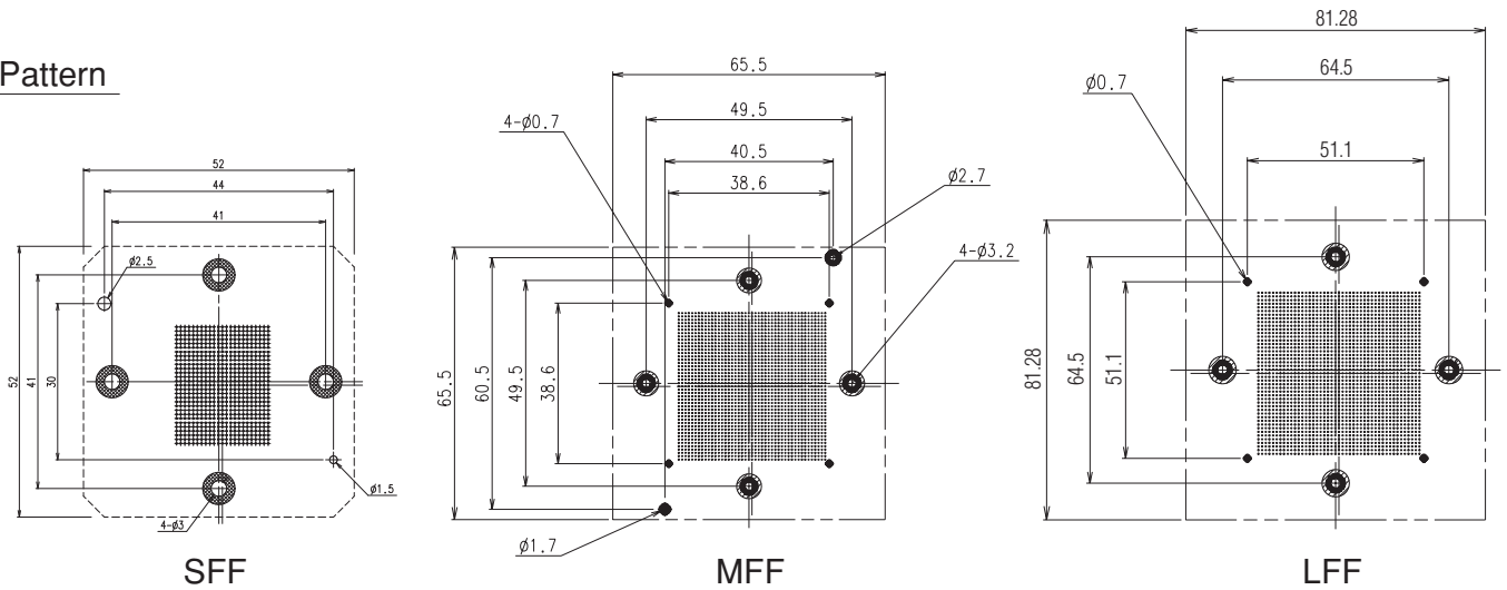
OTL/OTB versatile socket for small size (10-25mm PKG)
