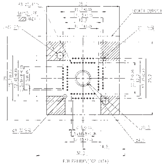
QFN-68H-0.5-02
